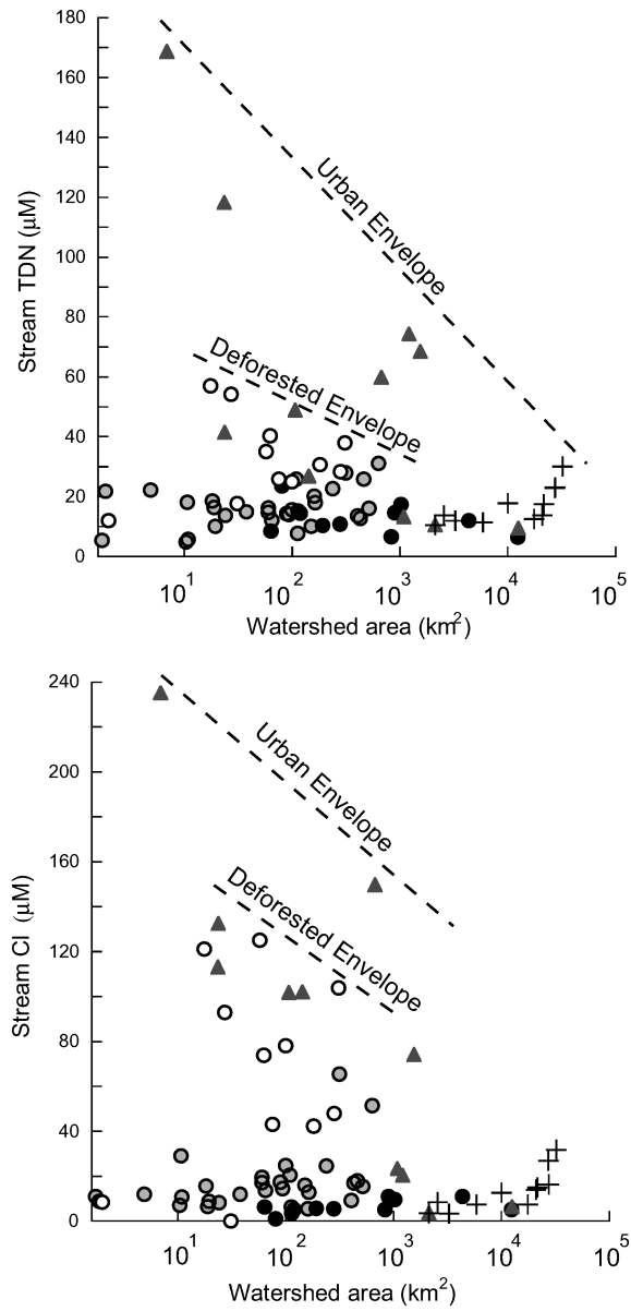
Figure 6. Chloride and TDN concentrations in stream water versus watershed area, dry season only. Symbols as in Figures 2 and 5. The urban envelope indicates the maximum concentrations observed for watersheds with urban population density greater than 5 persons per \text{km}^2 . '+' signs indicate samples from the Ji-Paraná transect.
